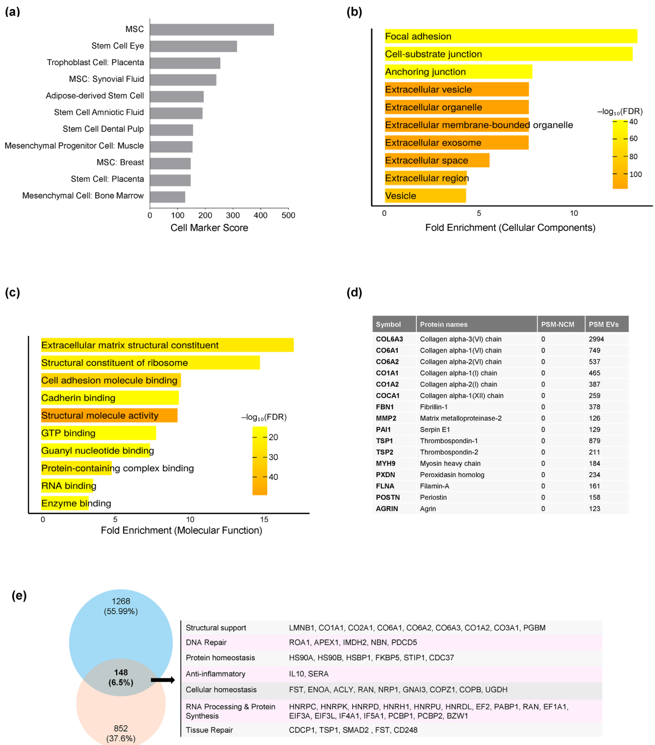
FIGURE 5 | hTSC-CM and EVs are enriched in proteins downregulated in senescence. (a) CellMarker analysis of the proteome of hTSC-EVs, showing general enrichment in stem cells and confirming the stem cell origin of hTSCs. (b) GO enrichment analysis of hTSC-EV cellular components. (c) GO enrichment analysis of hTSC-EV molecular functions. (d) Mass spectrometry analysis of hTSC-EV protein composition, highlighting ECM-related and structural proteins. (e) Venn diagram of protein sets enriched in hTSC-CM and EVs (pink) and reduced in senescent cells (blue) (Munk et al. 2021); the intersection shows 148 shared proteins (Table S5) including the highlighted proteins, grouped by function.
