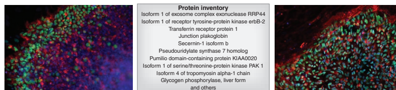
Figure 1 | A proteomic comparison of human ESCs and iPSCs. Images of iPSCs (left) and ESCs (right) are shown stained for Tra-1-60 (red), Oct-4 (green) and with 4',6-diamidino-2-phenylindole (DAPI). Though the proteome inventories of iPSCs and ESCs are similar, subtle yet substantial differences in protein expression and phosphorylation were found for a number of proteins. Images courtesy of Jordan Pomeroy, Pera laboratory.
